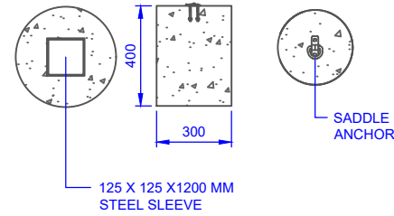
ANCHOR FOOTING B (X10) (F2)
