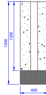
POLE FOOTING A (X3) (F1) FOR SOIL TYPES S, M
