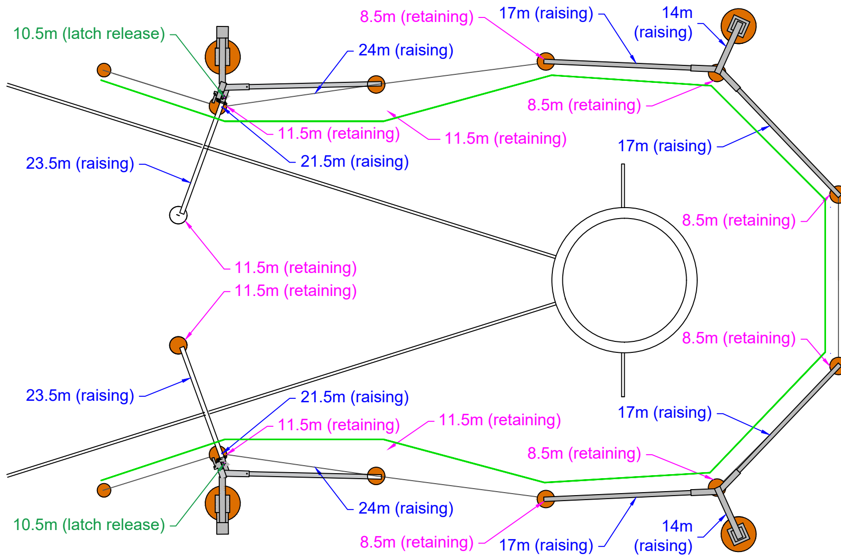
ROPE LOCATIONS
